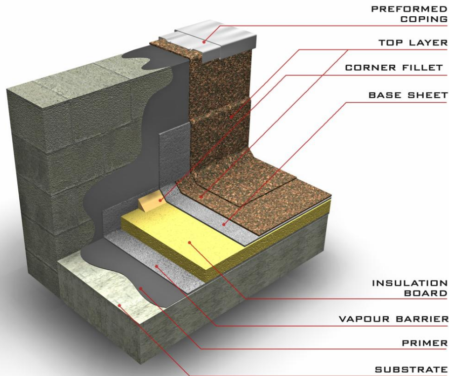
Figure 1 – Parapet Wall with Coping Detail
