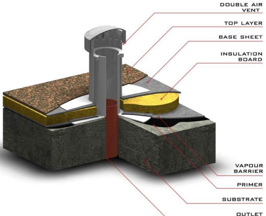
Figure 2 - Vent Pipe Penetration Detail
